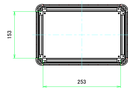
C-C (1:5)
